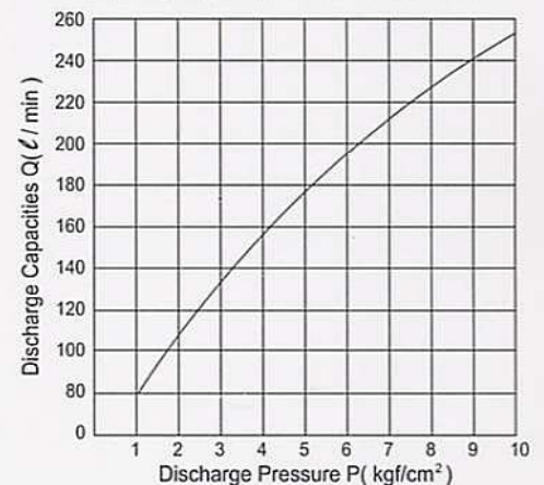
Discharge Capacities Performance Curve Chart
