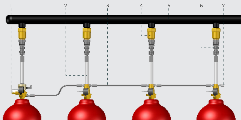
Master and Slave Cylinder Front View
