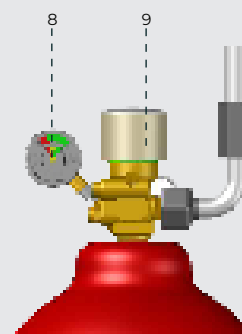
Master Side View
