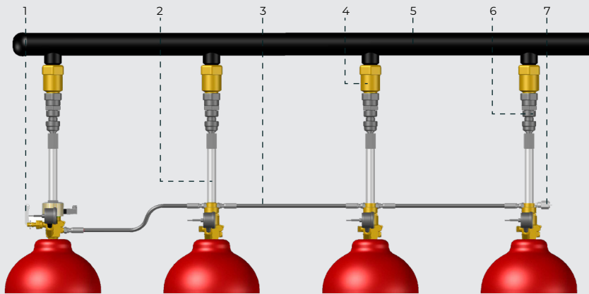
Master and Slave Cylinder Front View
